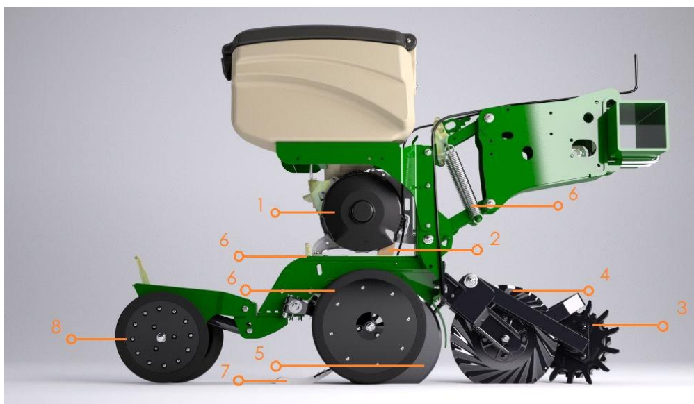
Fig. 1. Section of the seeder of precision seeding: 1 – construction of the seeding device, 2 – valve, 3 – unfolders, 4 – turbodisc, 5 – opener, 6 – sowing depth adjustment system, 7 – seed sealer, 8 – rolling wheels
