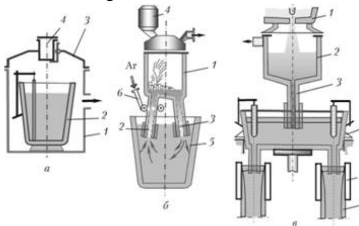
Figure 1 – Vacuum degassing process
