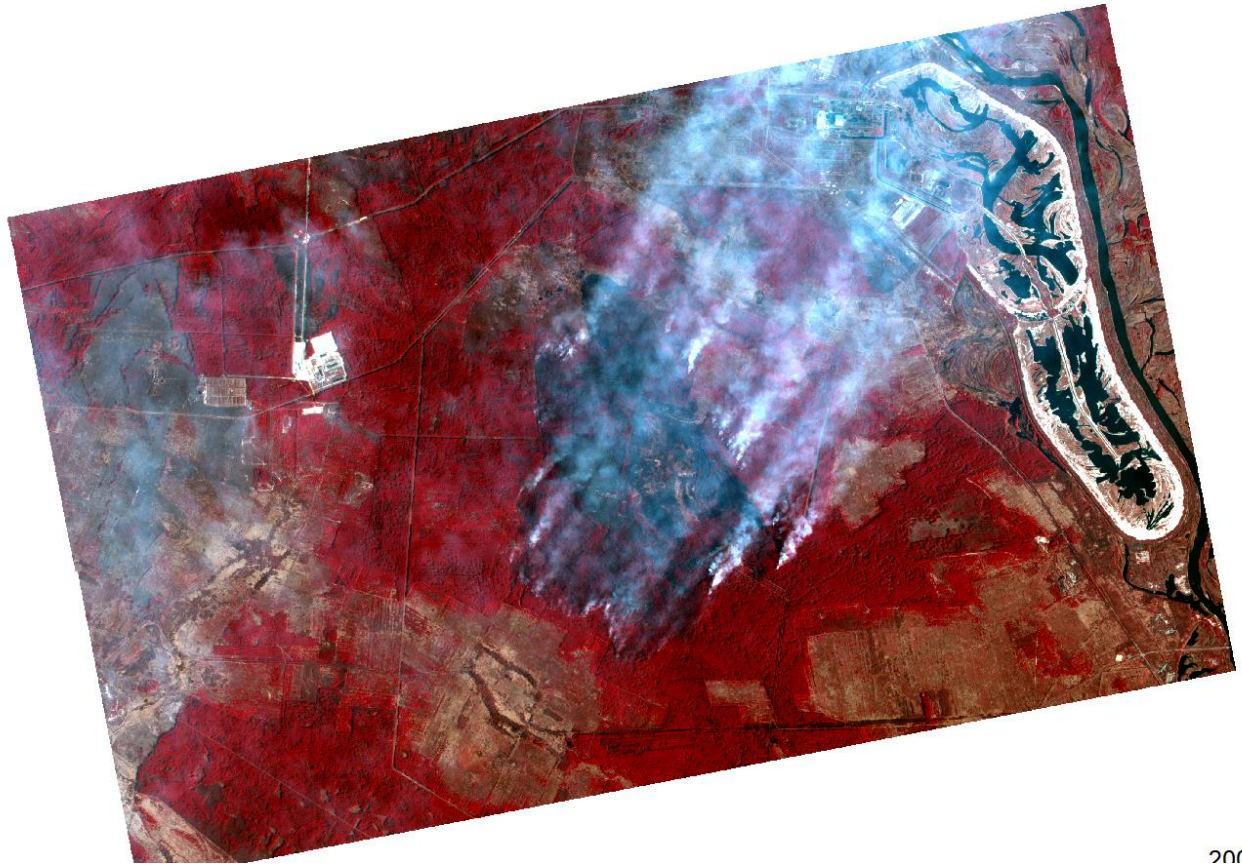
Fig. Large forest fire occurred 8-th of April 2020 in close vicinity of Red Forest in 10-km zone of the Chernobyl Exclusion Zone. Smoke is moving toward Belorussia. Preliminary assessment shows burned area at least 2000 ha. Image: PlanetScope, acquisition date and time 2020-04-09 T06:21:33
