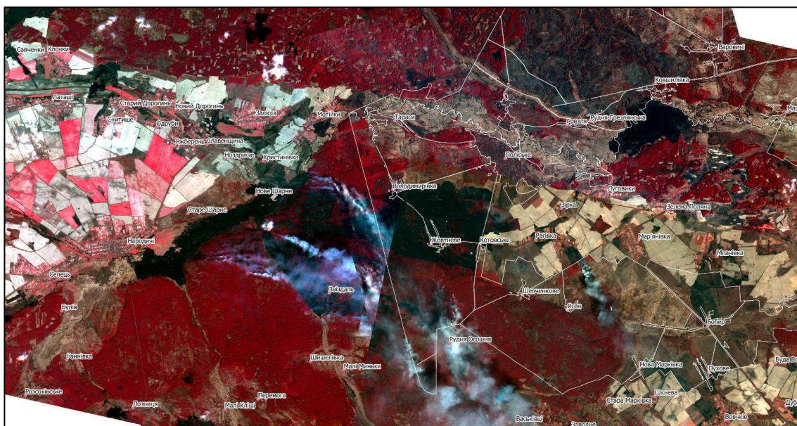
Fig. 3. Composite Planet satellite image of the fire development on the territory of the western part of the CEZ, 3-5 April 2020. Image: PlanetScope.
