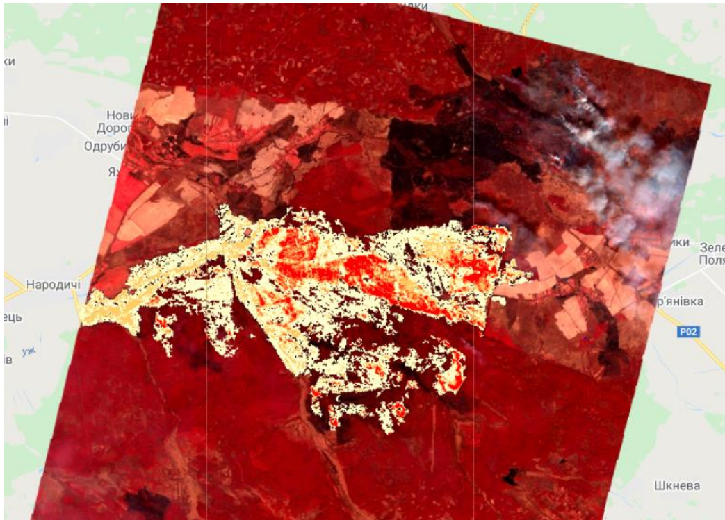
Fig. Fire that is burning near Narodychy - Poleskii cities in the western part of the Chernobyl Exclusion Zone. By 10th of April total area reached up to 12 000 ha. Image: PlanetScope, acquisition date and time 2020-04-08 T09:08:30
