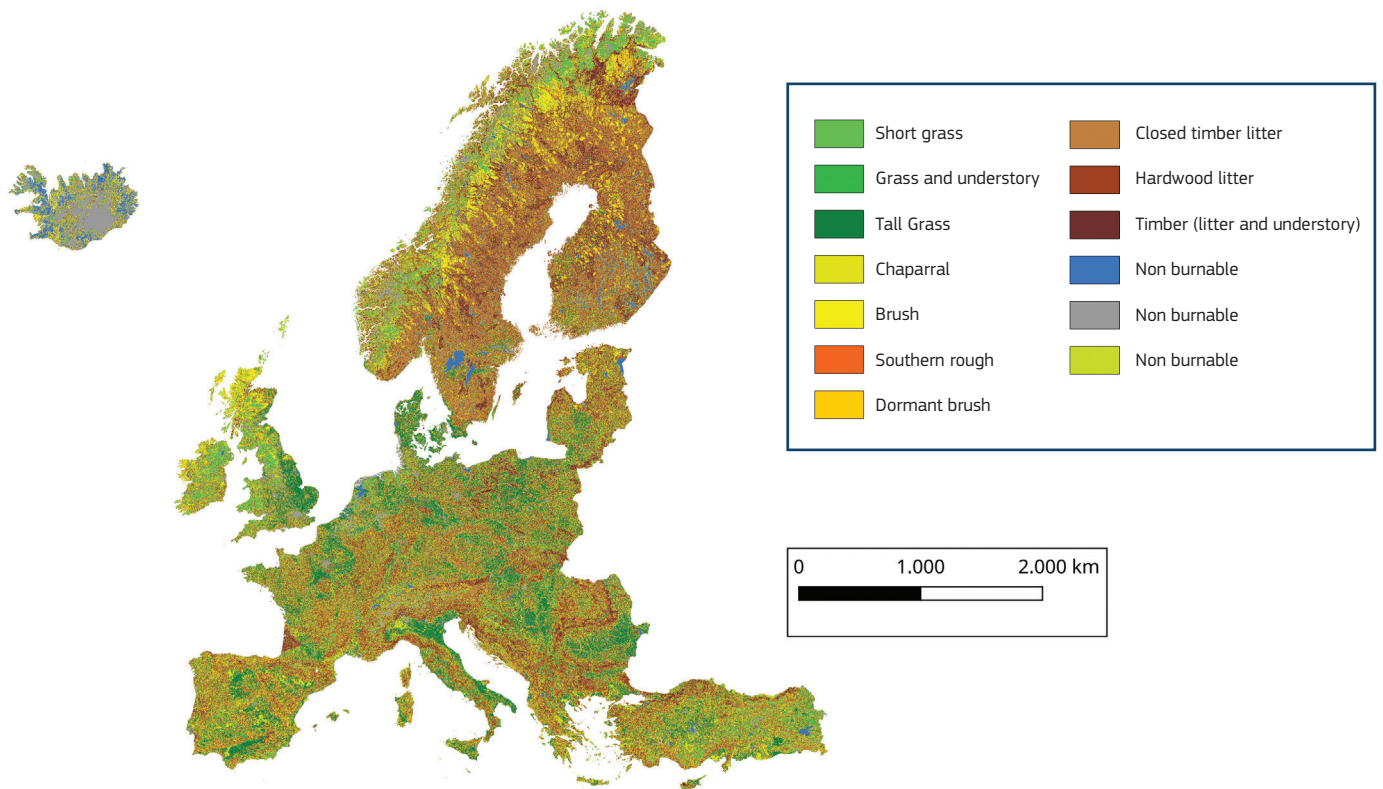
Figure 4: EFFIS Fuel distribution in Europe
