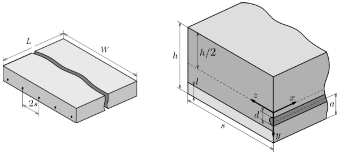
Fig. 1. The cross-section of plate (on left) and one of plate period (on right)
