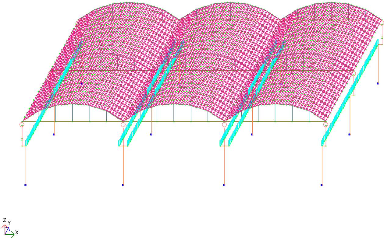
Fig. 3. Design scheme of the frame in the spatial version
