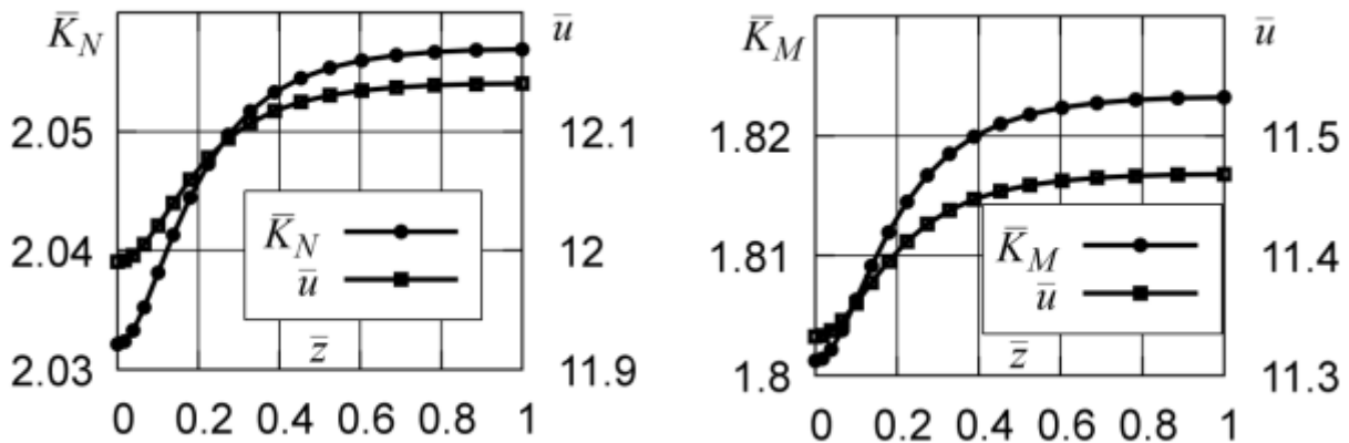
Fig. 2. The distributions of dimensionless SIF ( \bar{K} ) and openings ( \bar{u} ) in pure tension (on left) and pure bending (on right) of the plate
