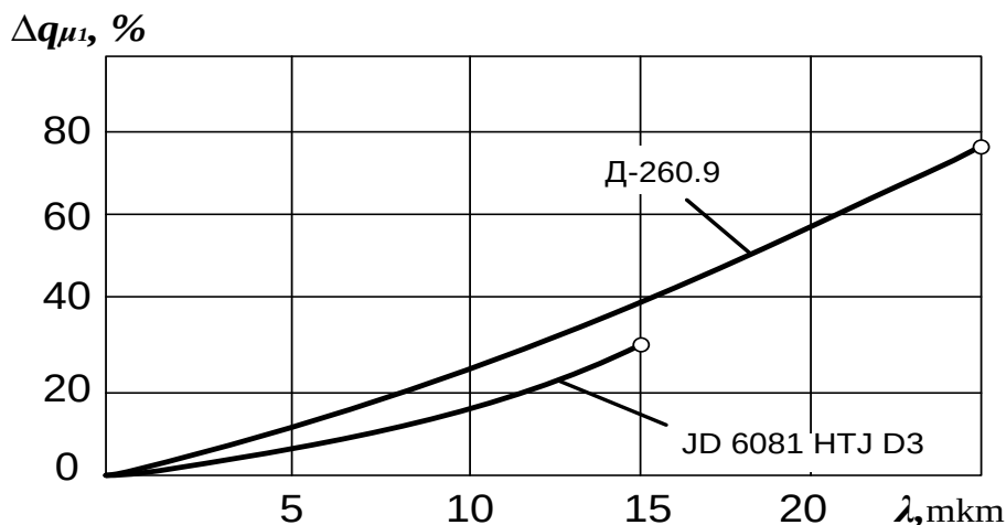
Fig. 4. – The dependence of the reduction of the cyclic fuel supply \Delta q_{\mu} on the screening density \lambda of the filter
